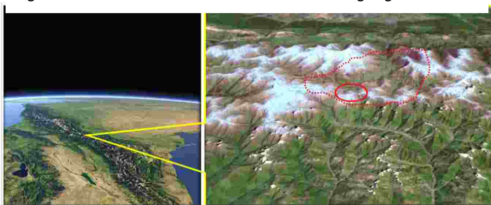
Figure.1 Central Great Caucasus. Location of the Kazbegi region
