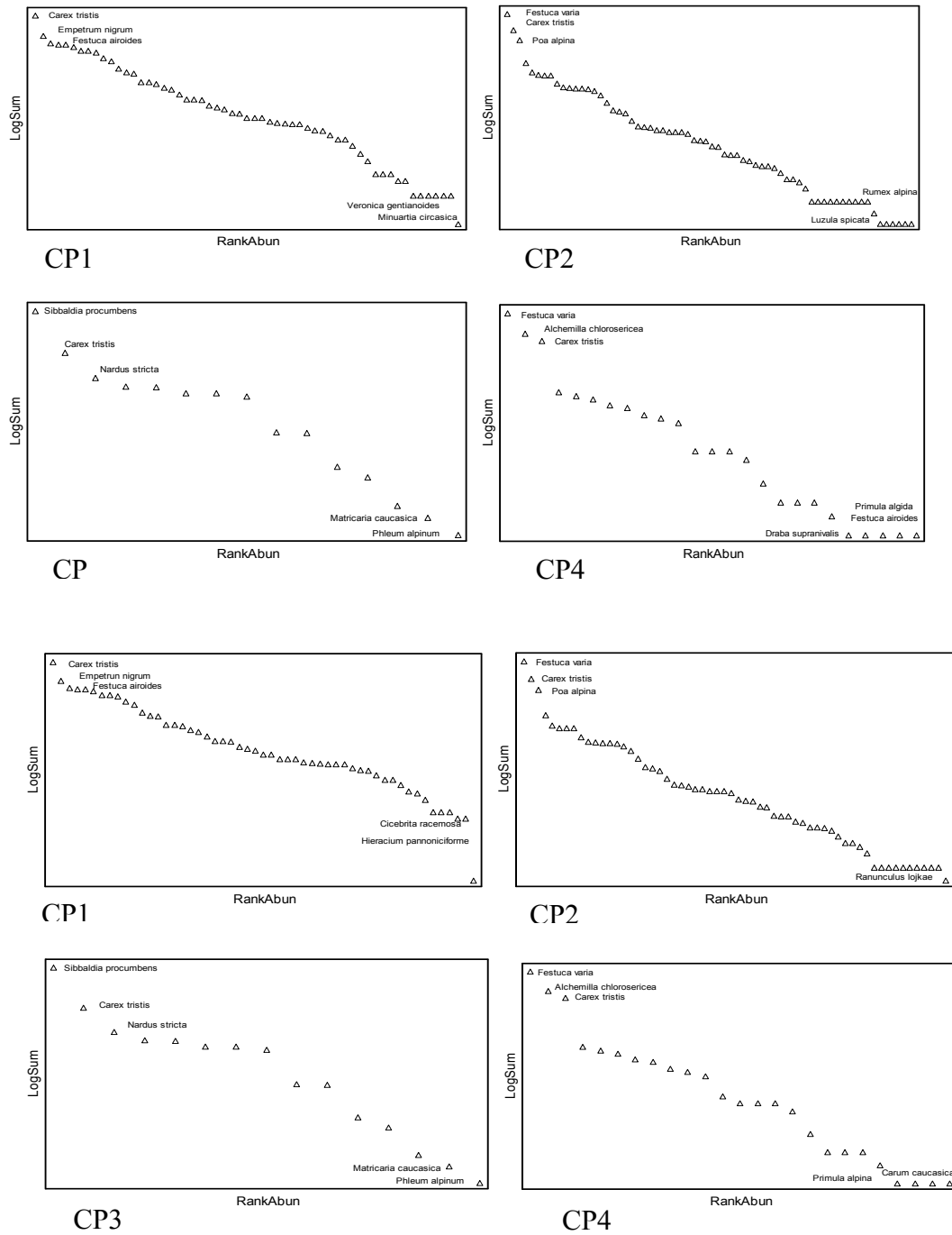
Figure 10. Dominance Curve Test.. Rank abundance of species in all summit (CP1, CP2, CP3, CP4) in 2001 (A) and 2008 (B)
